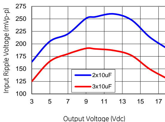
Figure 29. Input ripple voltage for various output voltages with 2x10 \mu F or 3x10 \mu F ceramic capacitors at the input (maximum load). Input voltage is 28V.
