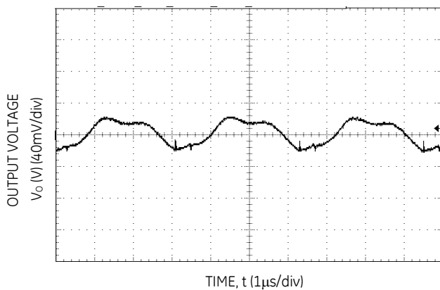
Figure 3. Typical output ripple and noise ( V_{IN} = 28\text{V} , I_o = I_{o,max} ).
