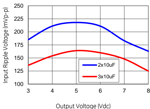
Figure 28. Input ripple voltage for various output voltages with 2x10 \mu F or 3x10 \mu F ceramic capacitors at the input (maximum load). Input voltage is 12V.
