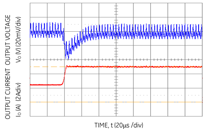
Figure 4. Transient Response to Dynamic Load Change from 50% to 100% at 28V_{in} , C_{ext} = 10\mu\text{F} ceramic + 330\mu\text{F} polymer, C_{Tune}=10\text{nF} & R_{Tune}=150\Omega
