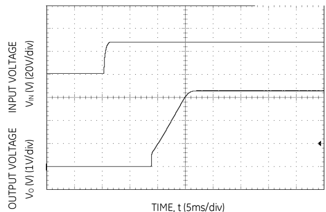
Figure 6. Typical Start-up Using Input Voltage ( V_{IN} = 28\text{V} , I_o = I_{o,max} ).
