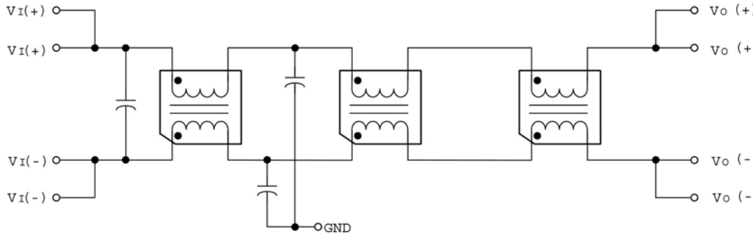
Figure 4. Internal Schematic
