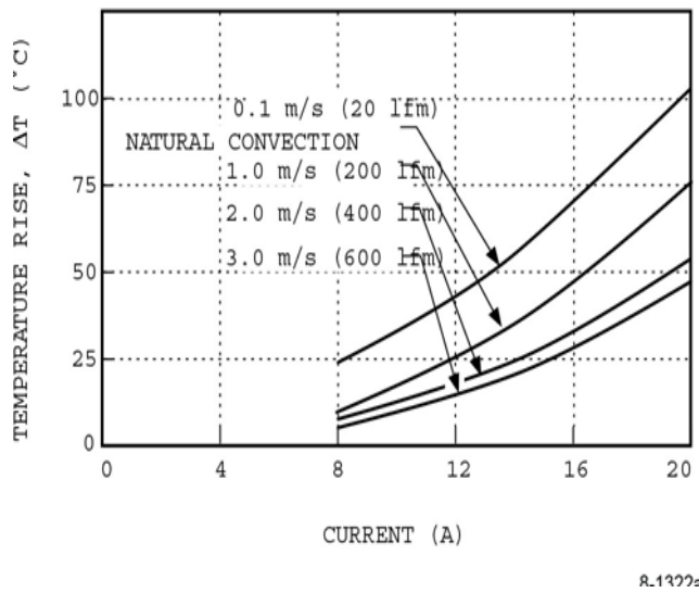
Figure 1. Typical Case Temperature Rise vs. Average Current (Case Temperature Must Be Kept Below 100 ^{\circ}\text{C} )
