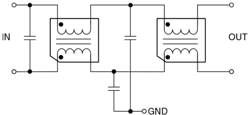
Figure 5. Internal Schematic
