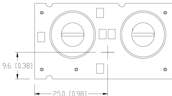
Figure 14: Pick and Place Location.
