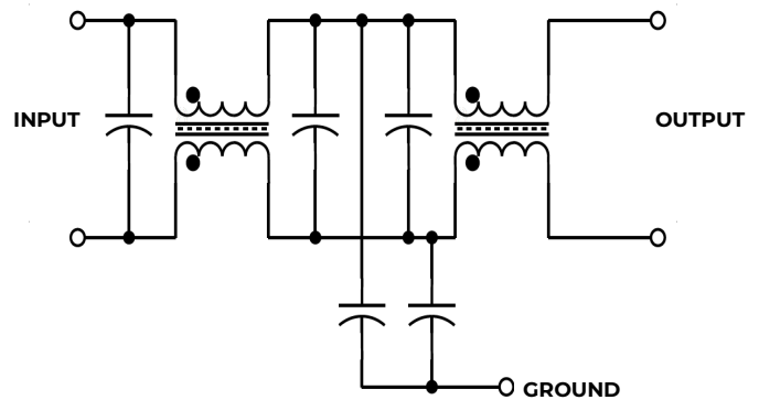
Figure 6: Internal Schematic
