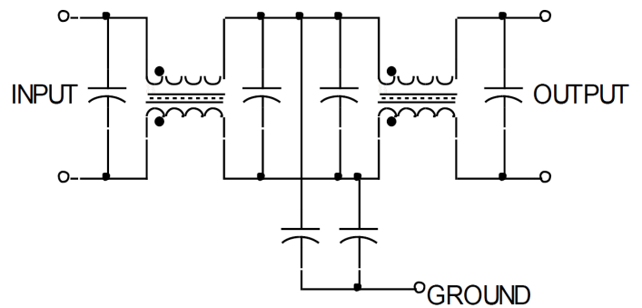
Figure 4: Internal Schematic
