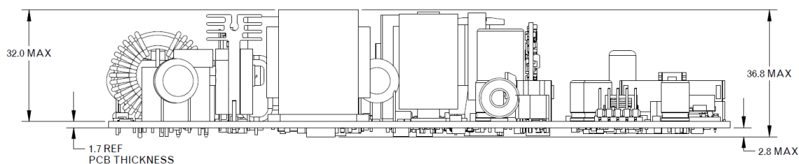
SIDE VIEW
