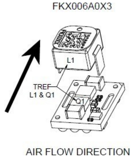
Figure 47. Preferred airflow direction and location of hotspots of the module ( T_{ref} ).
