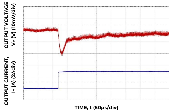
Figure 4. Transient Response to Dynamic Load Change from 5% to 100% at 12 V in , C out – 2x 330μF, 6x 100μF, C tune - 10μF, R tune – 500
