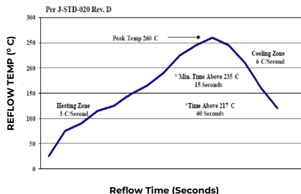
Figure 48. Recommended linear reflow profile using Sn/Ag/Cu solder.
