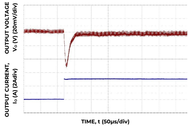
Figure 22. Transient Response to Dynamic Load Change from 50% to 100% at 12V in , C out =5x100μF, C tune =3.3nF, R tune = 500
