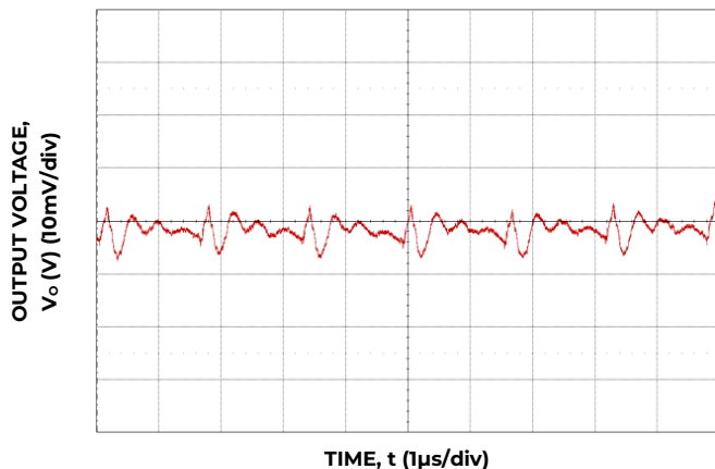
Figure 3. Typical Output Ripple and Noise, (C o = 88 μF Ceramic, V IN = 12 V, I o = I o, max .)
