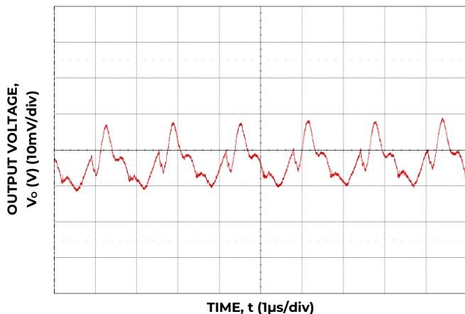
Figure 33. Typical Output Ripple and Noise, (C o = 88 μF Ceramic, V IN = 12 V, I o = I o, max .)
