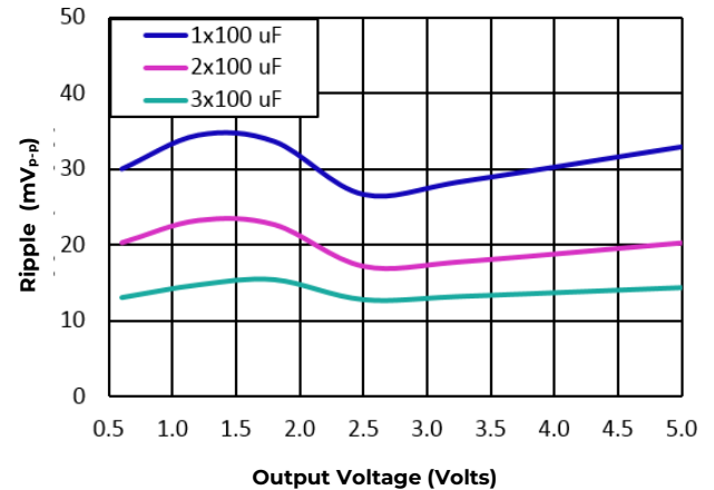
Figure 38. Output ripple voltage for various output voltages with external 1x100 \mu F, 2x100 \mu F, and 3x100 \mu F ceramic capacitors at the output (6A load). Input voltage is 12V.
