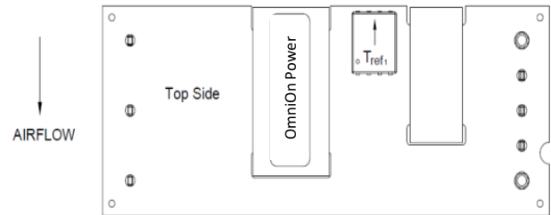
Figure 13a. T_{ref1} Temperature Measurement Location for Open Frame Module.
