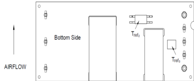
Figure 13b. T_{ref2} and T_{ref3} Temperature Measurement Locations for Open Frame Module.
