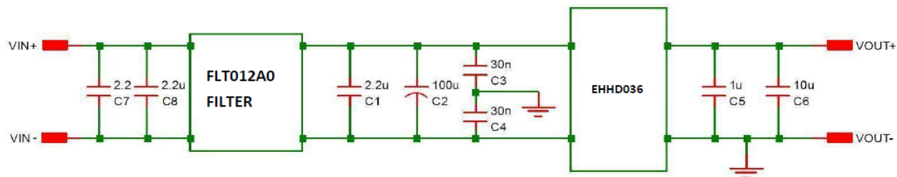
Figure 27. EMC Considerations
