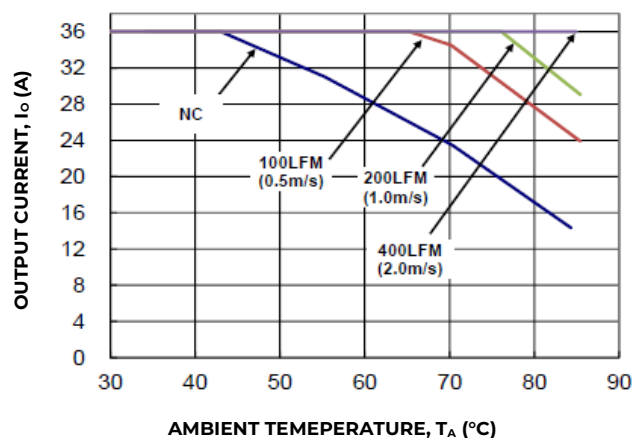
Figure 20. Output Current Derating for the Module with—18 Heatplate; Airflow in the Transverse Direction from V_{out}(-) to V_{out}(+) ; V_{IN}=24V , V_O=3.3V .
