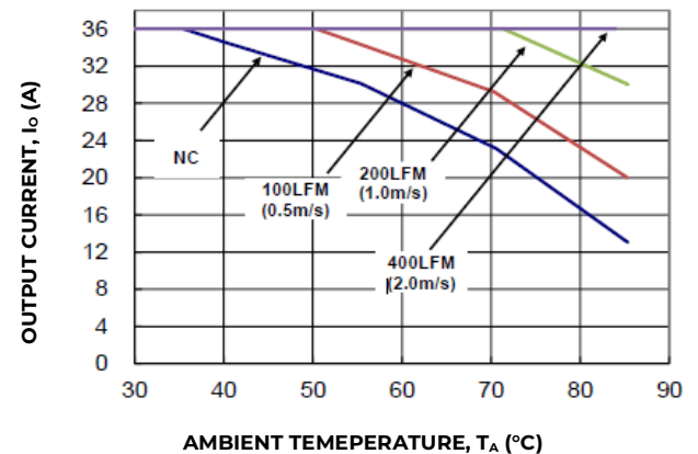
Figure 18. Output Current Derating for the Open Frame Module; Airflow in the Transverse Direction from V_{out}(-) to V_{out}(+) ; V_{IN}=24V , V_O=3.3V .
