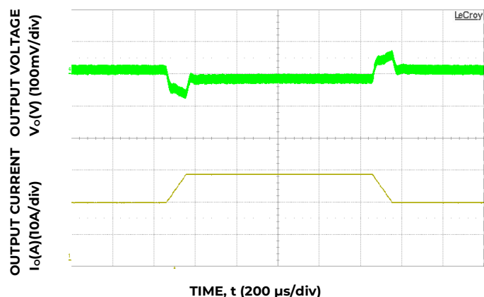
Figure 3. Transient Response to 0.1A/μs Dynamic Load Change from 50% to 75% to 50% of full load, V_{in}=24V
