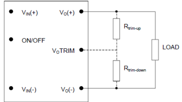
Figure 12. Circuit Configuration to Trim Output Voltage.
