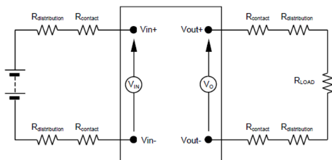
NOTE: Figure 9. Output Voltage and Efficiency Test Setup. All
