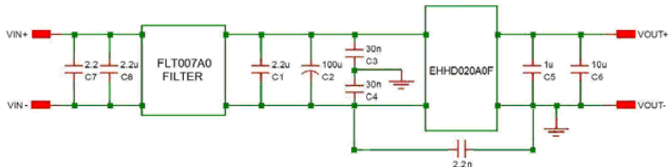
Figure 28. EMC Considerations
