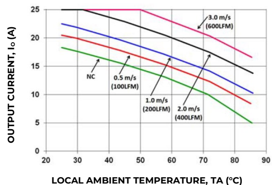
Figure 20. Output Current Derating for the Open Frame EBW025A0B in the Transverse Orientation; Airflow Direction from V_{in}(-) to V_{in}(+) ; V_{in} = 48 V.
