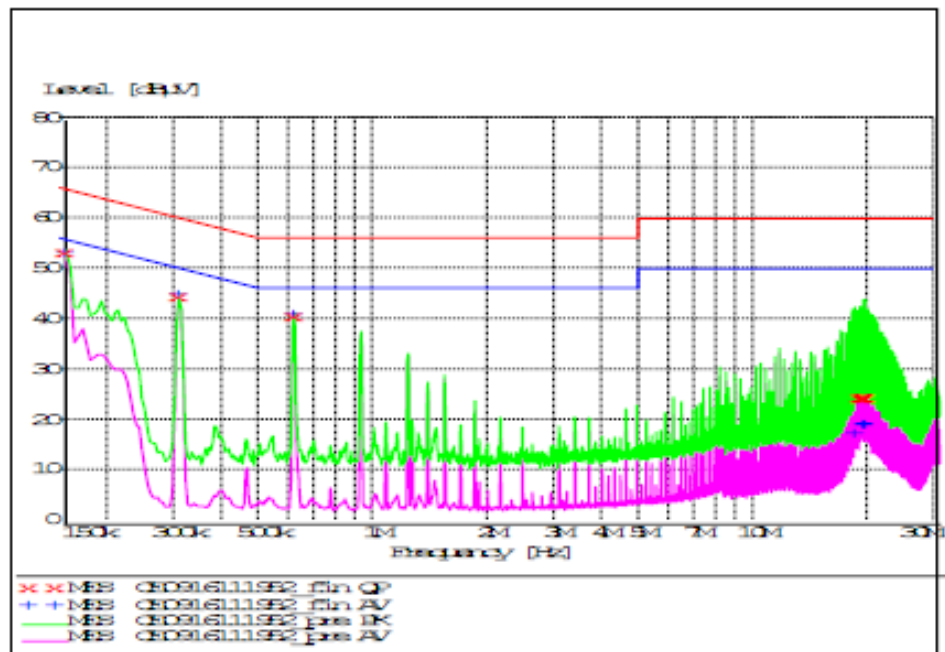
Figure 24. EMC Considerations.
