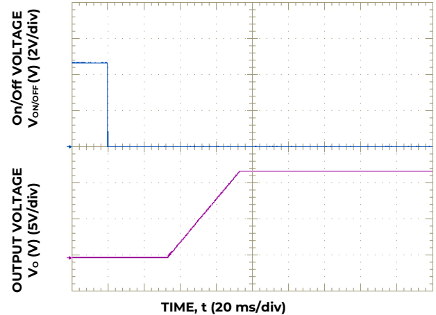
Figure 4. Typical Start-Up Using Remote On/Off with V_{in} applied, negative logic version shown.
