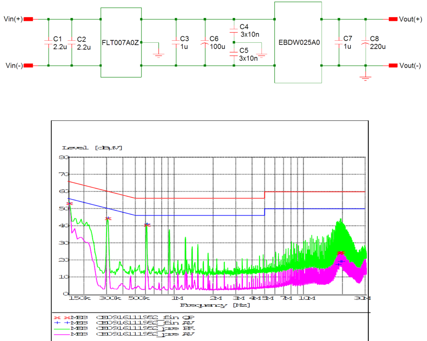
Figure 24. EMC Considerations
