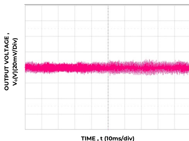
Figure 6. 5V DC output ripple and noise, full load, V_{IN} = 185V_{AC} , 20MHz bandwidth
