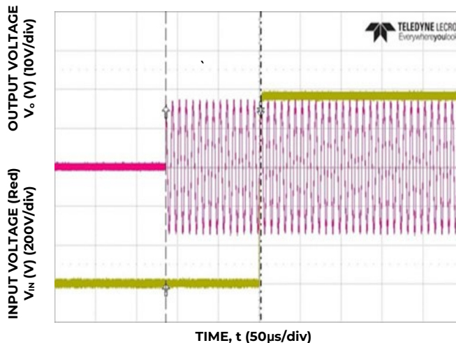
Figure 5: Typical Start-up ( V_{IN} = 230V , Full Load)
