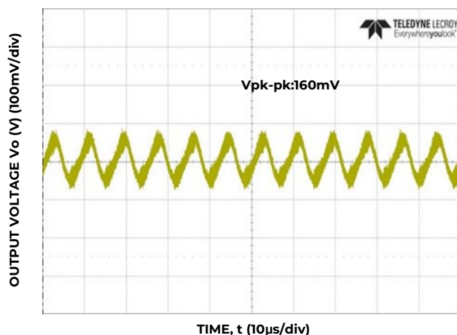
Figure 2: Typical output ripple and noise ( V_{IN} = 230V_{ac} , 100% load)
