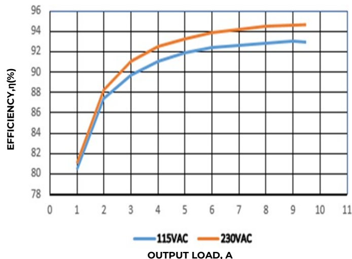
Figure 1: Power Supply Efficiency Versus Output Current
