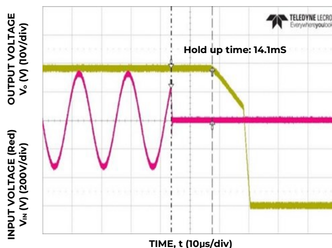
Figure 7. Typical Hold-up Waveforms ( V_{IN} = 230V , 100% Load)
