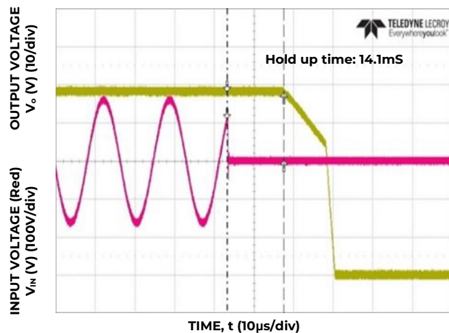
Figure 6. Typical Hold-up Waveforms ( V_{IN} = 115V_{ac} , 100% Load)
