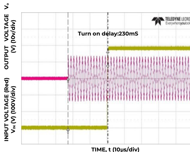
Figure 4: Typical Start-up ( V_{IN} = 90V_{ac} , Full Load)
