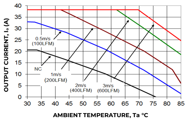
Figure 2. Power Data shown for model CLP0412FPXXXZ03A, 115V AC in. At 230VAC in derating is the same or better. Standby output is loaded at 0.25A. For derating at other input voltages and other models, consult the OmniOn Technical representative.
