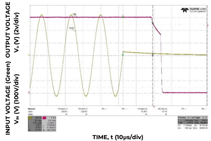
TIME, t (10μs/div) Figure 8. Typical Hold-up ( V_{IN} = 230V, 100% Load)
