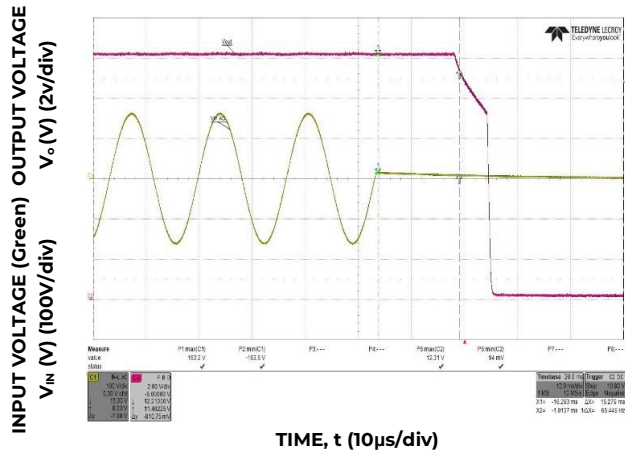
TIME, t (10μs/div) Figure 7. Typical Hold-up ( V_{IN} = 115V, 100% Load)
