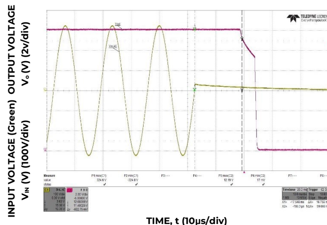
Figure 8. Typical Hold-up ( V_{IN} = 230V , 100% Load)
