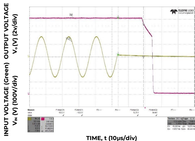
Figure 7. Typical Hold-up ( V_{IN} = 115V , 100% Load)
