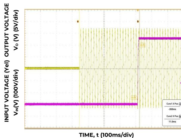
Figure 6. Typical Start-up (V IN = 230V ac , Full load)
