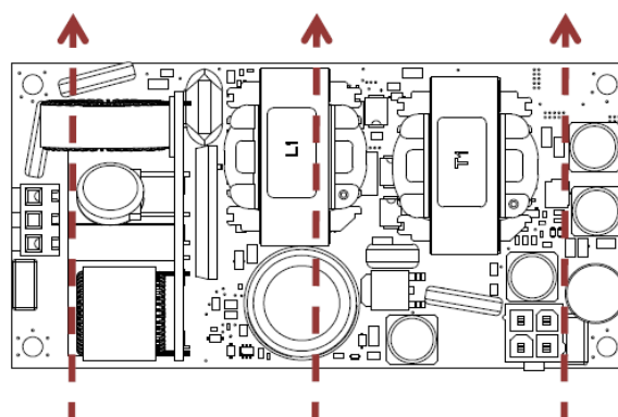
Fig. 10. Preferred airflow direction for cooling.
