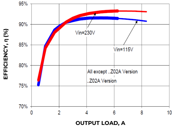
Figure 1. Power Supply Efficiency versus Output Current.
