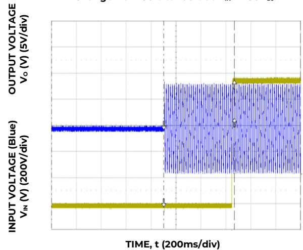
Figure 6. Typical Start-up ( V_{IN} = 230V_{ac} , Full load).
