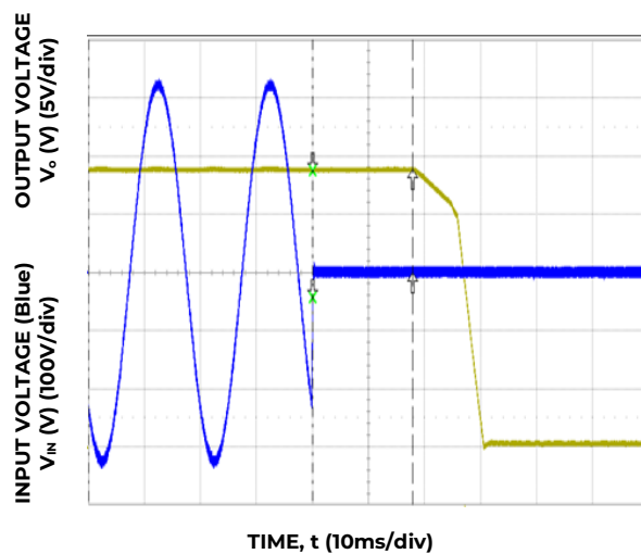
Figure 10. Typical Hold-up waveforms – ..Z02A version ( V_{IN} = 230V , 100% load).
