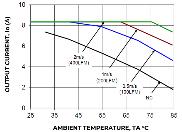
Figure 2. Derating Output Current versus Ambient Temperature and Airflow. Data shown for 115VAC in, at 230VAC in derating is the same or better. For derating at other input voltages, consult the OmniOn Technical representative.
