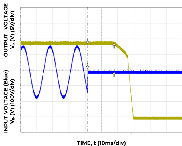
Figure 7. Typical Hold-up waveforms – all except ..Z02A version ( V_{IN} = 115V , 100% load).
