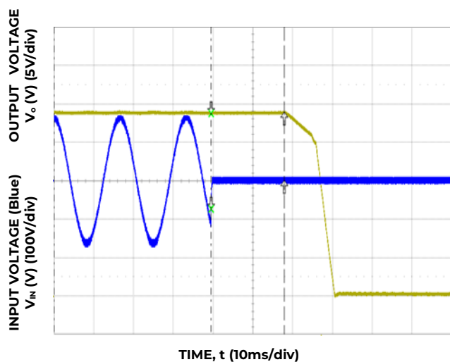
Figure 9. Typical Hold-up waveforms – ..Z02A version ( V_{IN} = 115V , 100% load).
