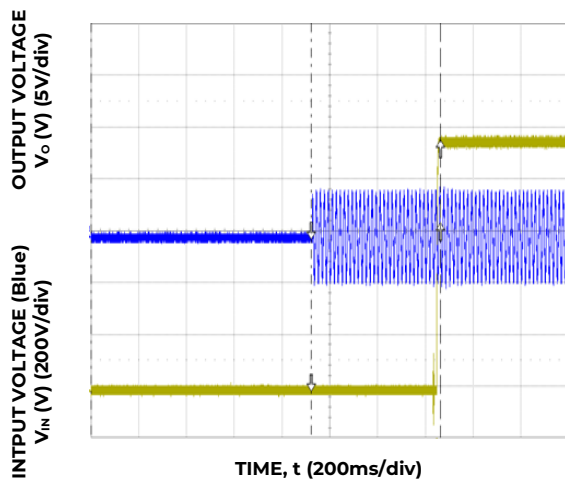
Figure 5. Typical Start-up ( V_{IN} = 115V_{ac} , Full Load).
