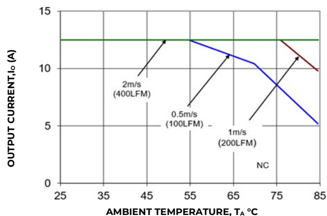
Figure 2. Derating Output Current versus Ambient Temperature and Airflow. Data shown for 115V AC in, at 230V AC in derating is the same or better. For derating at other input voltages, consult the OmniOn Technical representative.
