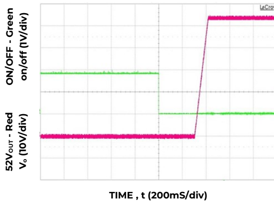
Figure 9. 52V DC soft start delay when ON/OFF is asserted, V IN =230V AC - I°C mode.
