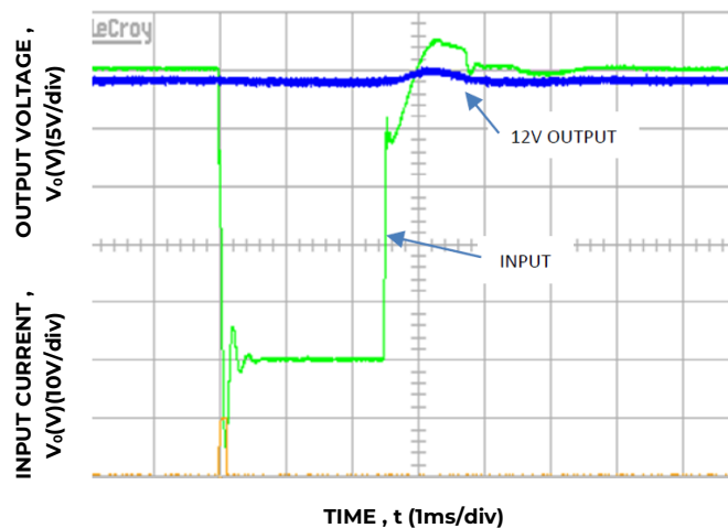
Figure 12. Ride through: full load V in = -48V DC
