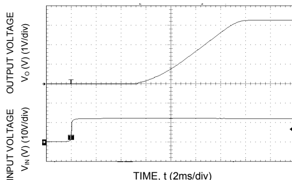
Figure 16. Typical Start-Up with application of V_{in} ( V_{in} = 12.0\text{Vdc} , V_o = 3.3\text{Vdc} , I_o = 3\text{A} ).
