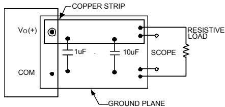
Figure 23. Input Reflected Ripple Current Test Setup.
