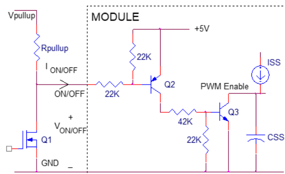
Figure 35. Circuit configuration for using positive On/Off logic.
