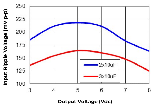
Figure 30. Input ripple voltage for various output voltages with 2x10 µF or 3x10 µF ceramic capacitors at the input (maximum load). Input voltage is 12V.
