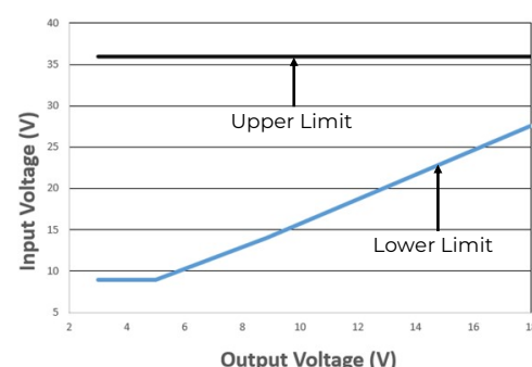
Figure 39. Output Voltage vs. Input Voltage Set Point Area plot showing limits where the output voltage can be set for different input voltages. (-78 version)
