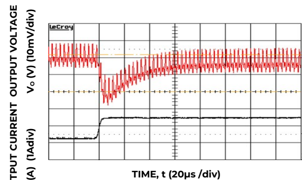
Figure 4. Transient Response to Dynamic Load Change from 50% to 100% at 28Vin, Cext - 10μF ceramic + 330μF polymer, CTune=5600pF & RTune=261Ω.
