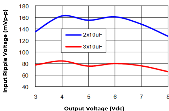
Figure 29. Input ripple voltage for various output voltages with 2x10 μF or 3x10 μF ceramic capacitors at the input (maximum load). Input voltage is 12V
