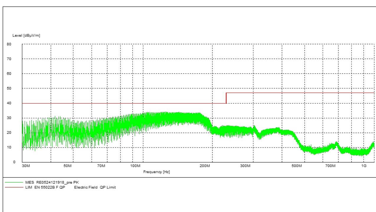
Figure 46. EMI Plot of APXW003 on evaluation board with 12 V in @ 1.2 A in / 5 Vdc @ 2.5 A out
