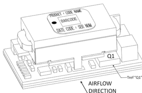
Figure 44. Preferred airflow direction and location of hot-spot of the module ( T_{ref} ).
