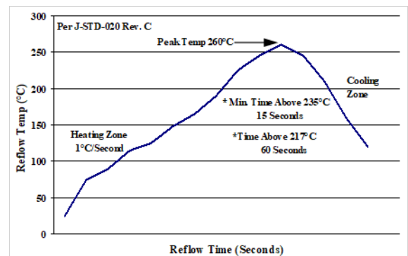
Figure 45. Recommended linear reflow profile using Sn/Ag/Cu solder.
