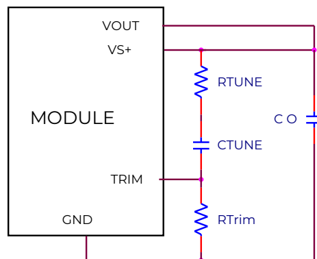
Figure 42. Circuit diagram showing connection of R_{TUNE} and C_{TUNE} to tune the control loop of the module.
