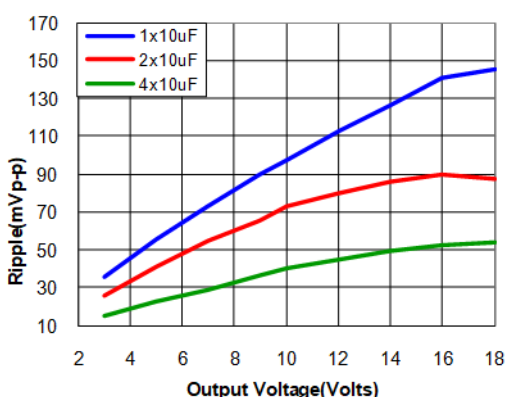
Figure 34. Output ripple voltage for various output voltages with external 1x10 µF, 2x10 µF or 4x10 µF ceramic capacitors at the output (max load). Input voltage is 28V
