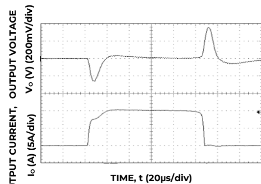
Figure 10. Transient Response to Dynamic Load Change from 50% to 100% of I_{O,max} .
