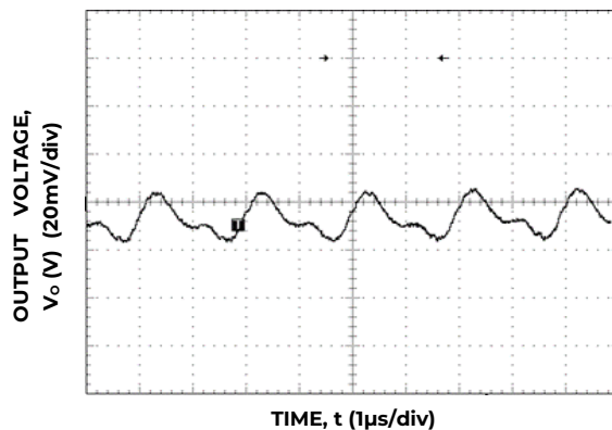
Figure 21. Typical Output ripple and noise, V_{IN} = 12 \text{ V} I_O = I_{O, \text{max.}}
