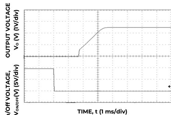
Figure 23. Typical Start-up Using On/Off Voltage ( I_O = I_{O, \text{max.}} )
