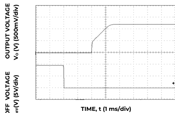
Figure 11. Typical Start-up Using On/Off Voltage ( I_O = I_{O,max} ).
