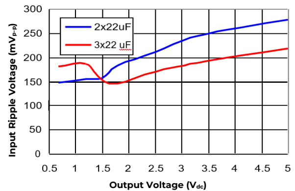
Figure 40. Input ripple voltage for various output voltages with 2x22\mu F or 3x22\mu F ceramic capacitors at the input (20A load). Input voltage is 12V
