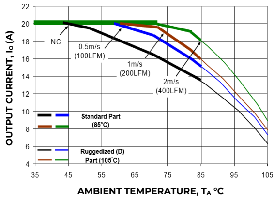
Figure 2. Derating Output Current versus Ambient Temperature and Airflow (Ruggedized Part is Discontinued)
