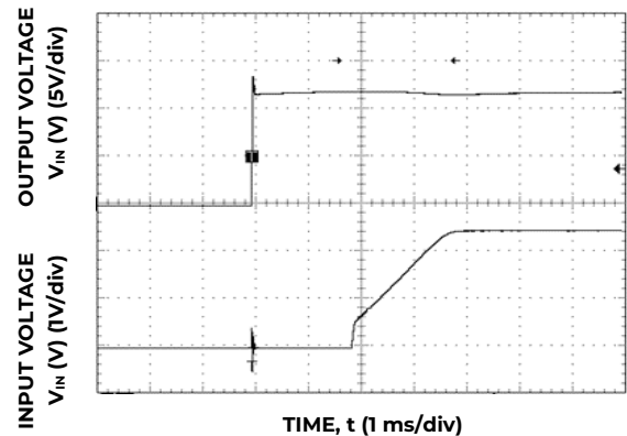
Figure 24. Typical Start-up Using Input Voltage ( V_{IN} = 12 \text{ V} , I_O = I_{O, \text{max.}} )
