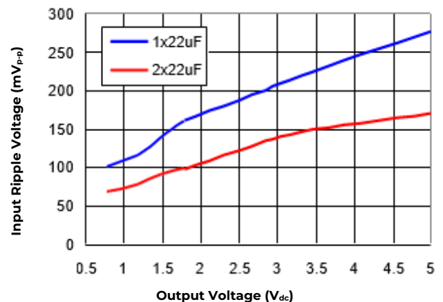
Figure 40. Input ripple voltage for various output voltages with 1x22\mu F or 2x22\mu F ceramic capacitors at the input (12A load). Input voltage is 12V.
