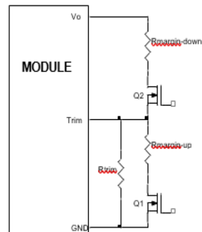
Figure 46. Circuit Configuration for margining Output voltage
