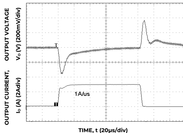
Figure 16. Transient Response to Dynamic Load Change from 50% to 0%.
