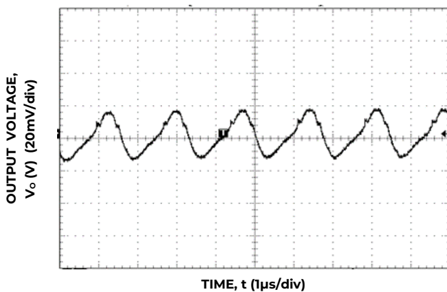
Figure 27. Typical output ripple and noise ( V_{IN} = 5V , I_o = I_{o,max} ).
