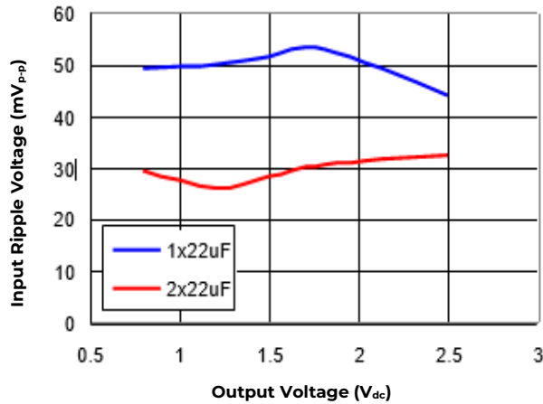
Figure 35. Input ripple voltage in mV, p-p for various output voltages with 1x22 μF or 2x22 μF ceramic capacitors at the input (3A load). Input voltage is 3.3V.
