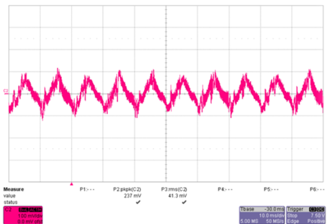
Figure 3. 48V DC output ripple and noise, full load, V_{IN}=230V_{AC} , 20MHz bandwidth
