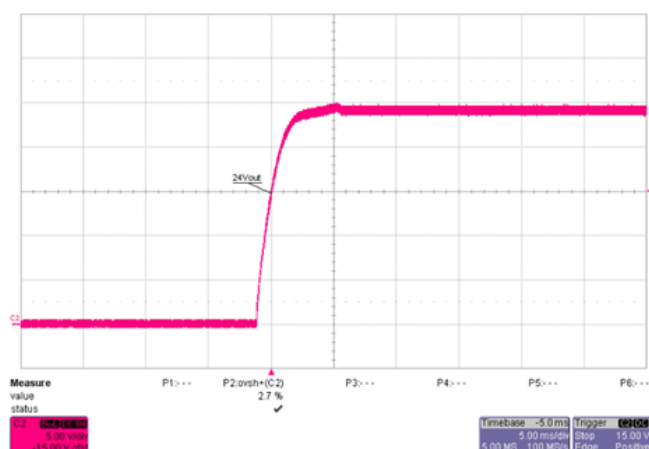
Figure 8. 24V DC soft start, full load, V N =230V AC
