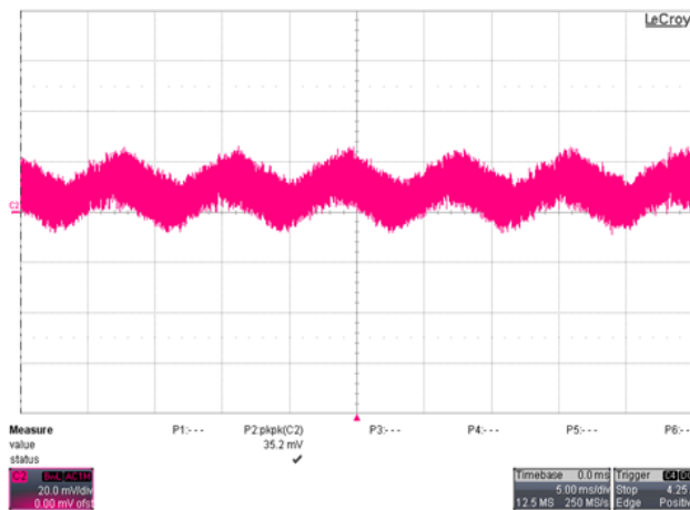
Figure 4. 24V DC output ripple and noise, full load, V_{IN}=230V_{AC} , 20MHz
