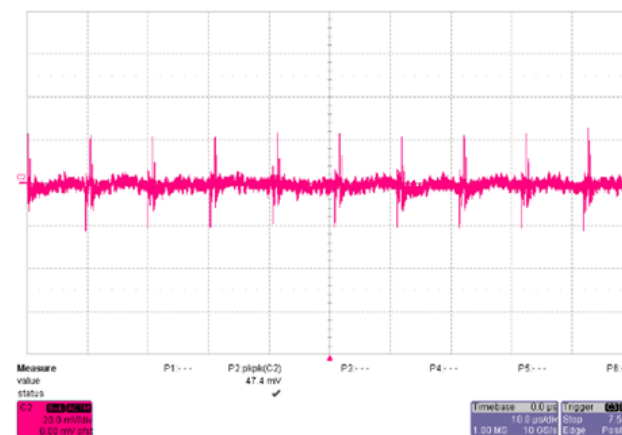
Figure 5. 5VSB output ripple and noise, full load, V_{IN}=230V_{AC} , 20MHz
