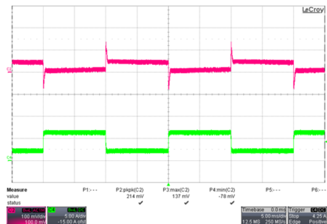
Figure 7. Transient response 24V DC load step 25% – 75%, V N = 230V AC
