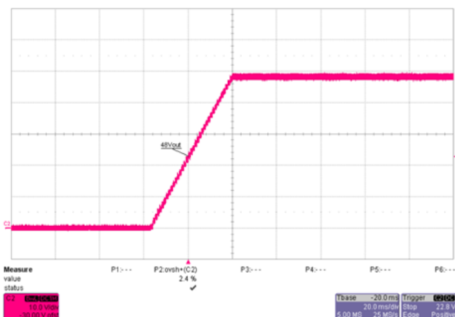
Figure 9. 48V DC soft start, full load, V N =230V AC
