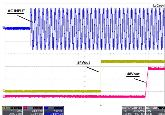
Figure 11. 24V DC & 48V DC turn on delay time, V N = 230V AC
