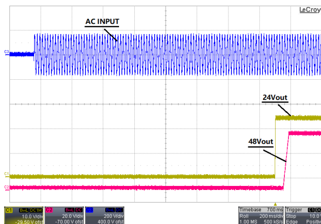
Figure 10. 24V DC & 48V DC turn on delay time, V N = 115V AC
