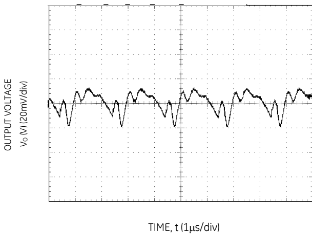
Figure 9. Typical output ripple and noise ( C_0=2 \times 47 \mu\text{F} ceramic, V_{IN} = 12\text{V} , I_o = I_{o,max} ).
