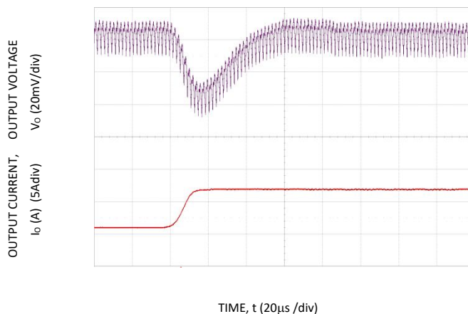
Figure 16. Transient Response to Dynamic Load Change on one output from 50% to 100% at 12Vin, C_{out} = 3 \times 47\mu F + 2 \times 330\mu F , C_{Tune} = 1800pF & R_{Tune} = 300\Omega
