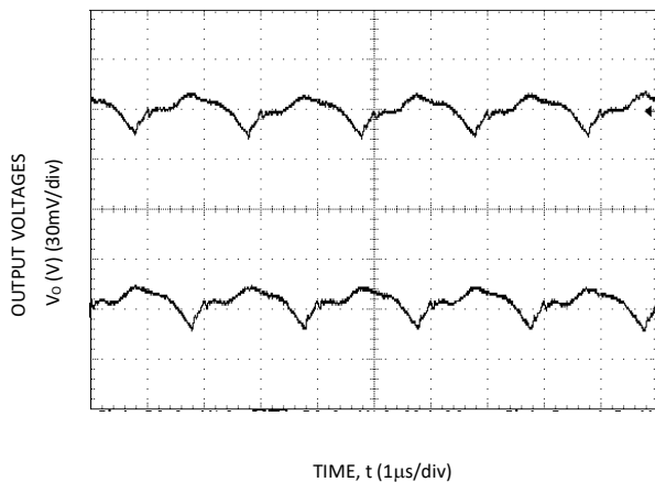
Figure 9. Typical output ripple and noise ( C_0 = 2 \times 0.1\mu\text{F} + 2 \times 47\mu\text{F} ceramic, V_{IN} = 12\text{V} , I_o = I_{o1,max}, I_{o2,max} ).
