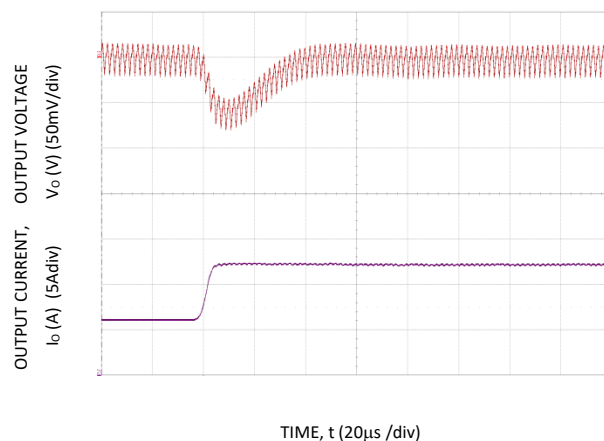
Figure 28 Transient Response to Dynamic Load Change on one output from 50% to 100% at 12V in , C_{out} = 3 \times 47\mu\text{F} + 1 \times 330\mu\text{F} , C_{Tune} = 1200\text{pF} & R_{Tune} = 300\Omega
