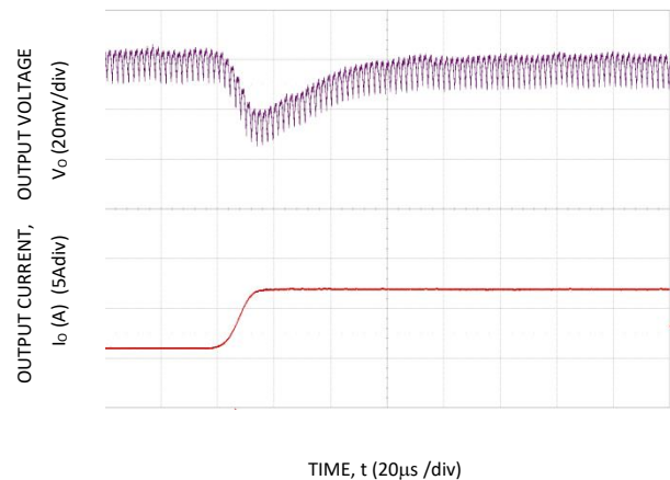
Figure 10. Transient Response to Dynamic Load Change on one output from 50% to 100% at 12V in , C_{out} = 3 \times 47\mu\text{F} + 3 \times 330\mu\text{F} , C_{Tune} = 2700\text{pF} & R_{Tune} = 300\Omega
