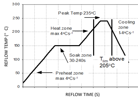
Figure 55. Time Limit, Tlim, Curve Above 205°C Reflow .
