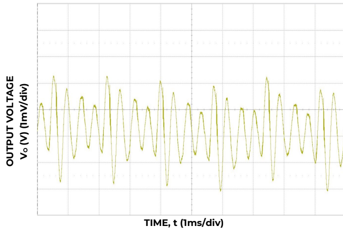
Figure 15. Typical output ripple ( C_o=4 \times 0.047\mu\text{F} + 4 \times 0.1\mu\text{F} + 15 \times 22\mu\text{F} +
