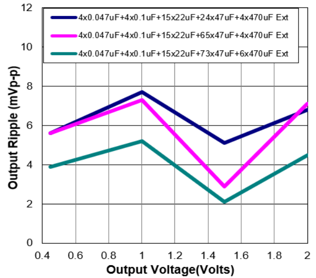
Figure 26. Peak to peak output ripple voltage for various output voltages with external capacitors at the output (160A load). Input voltage is 12V.
