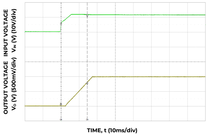
Figure 12. Typical Start-up Using Input Voltage ( V_{IN} = 12\text{V} , I_o = I_{o,max} ).
