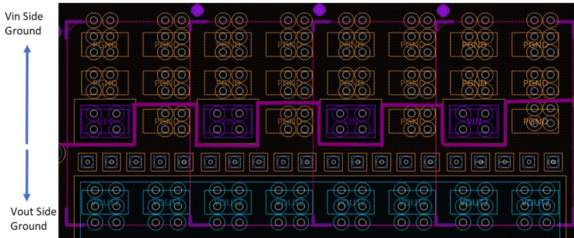
Figure 30. Example of split input-output ground
