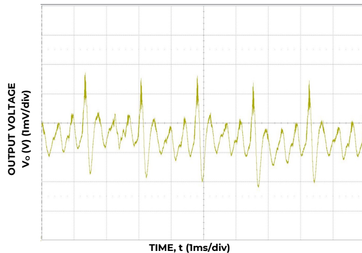
Figure 3. Typical output ripple ( C_o=4 \times 0.047\mu F + 4 \times 0.1\mu F + 15 \times 22\mu F + 73 \times 47\mu F + 6 \times 470\mu F polymer, V_{IN} = 12V , I_o = I_{o,max} ).
