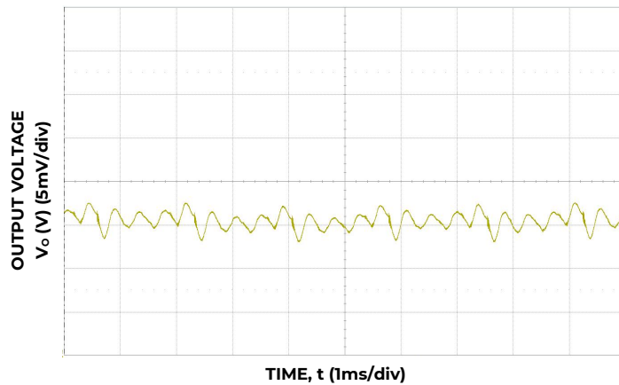
Figure 21. Typical output ripple ( C_o=4 \times 0.047\mu\text{F} + 4 \times 0.1\mu\text{F} + 15 \times 22\mu\text{F} + 73 \times 47\mu\text{F} + 6 \times 470\mu\text{F} polymer, V_{IN} = 12\text{V} , I_o = I_{o,max} )
