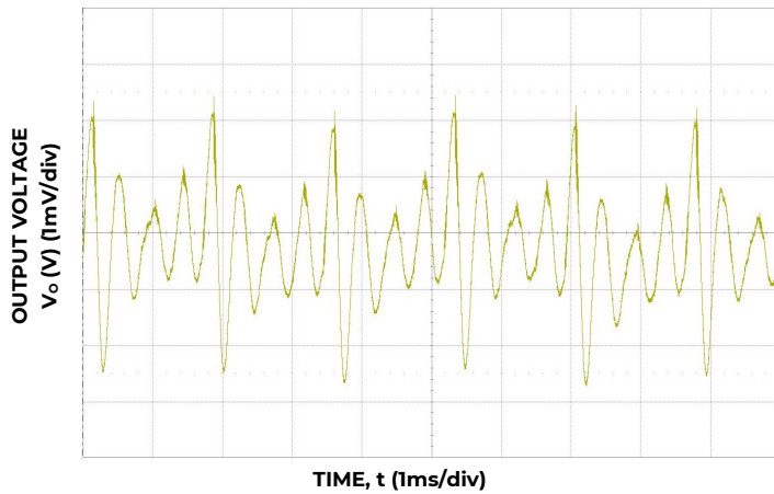
Figure 9. Typical output ripple( C_o=4 \times 0.047\mu\text{F} + 4 \times 0.1\mu\text{F} + 15 \times 22\mu\text{F} + 73 \times 47\mu\text{F} + 6 \times 470\mu\text{F} polymer, V_{IN} = 12\text{V} , I_o = I_{o,max} ).
