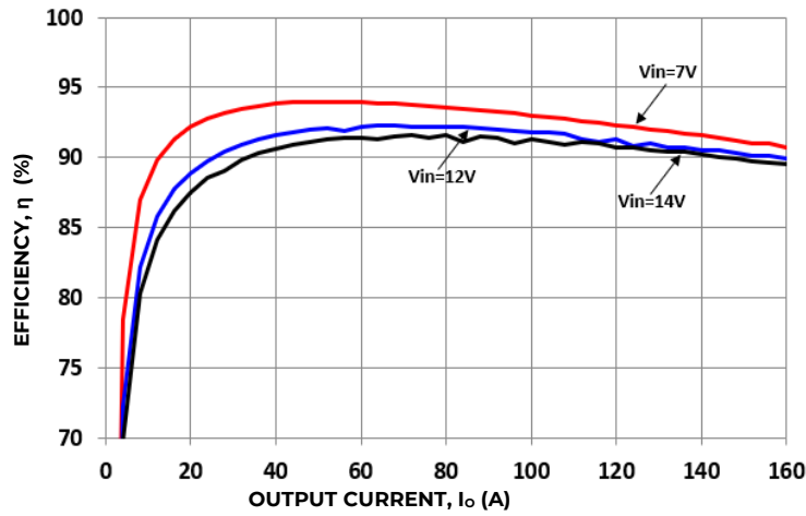
Figure 7. Converter Efficiency versus Output Current.
