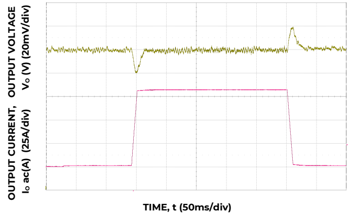
Figure 10. Trans. Resp. to 100A/μs Load Change from 25% to 75% at 12VIN, C_o=4 \times 0.047\mu\text{F} + 4 \times 0.1\mu\text{F} + 15 \times 22\mu\text{F} + 73 \times 47\mu\text{F} + 6 \times 470\mu\text{F} polymer
