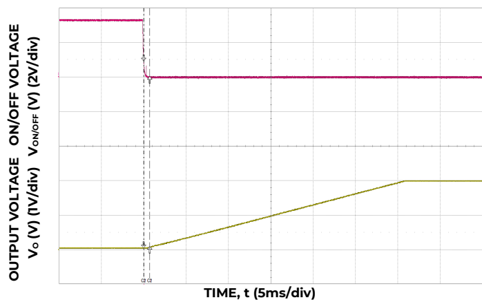
Figure 23. Typical Start-up Using On/Off Voltage ( I_o = I_{o,max} ).
