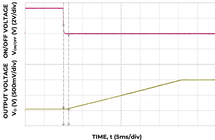
Figure 11. Typical Start-up Using On/Off Voltage ( I_o = I_{o,max} ).
