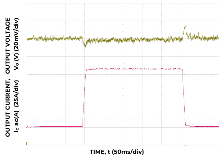
Figure 4. Trans. Resp. to 10A/μs Load Change from 25% to 75% at 12VIN, C_o=4 \times 0.047\mu F + 4 \times 0.1\mu F + 15 \times 22\mu F + 73 \times 47\mu F + 6 \times 470\mu F polymer
