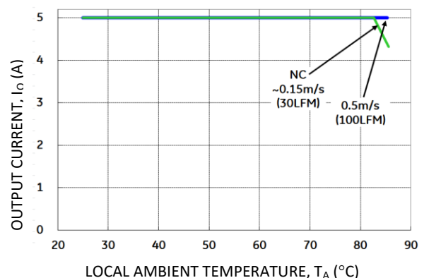
Figure 15. Output Current Derating for the Open Frame SHHD005A0F in the Transverse Orientation; Airflow Direction from Vin(-) to Vin(+); Vin = 48V.
