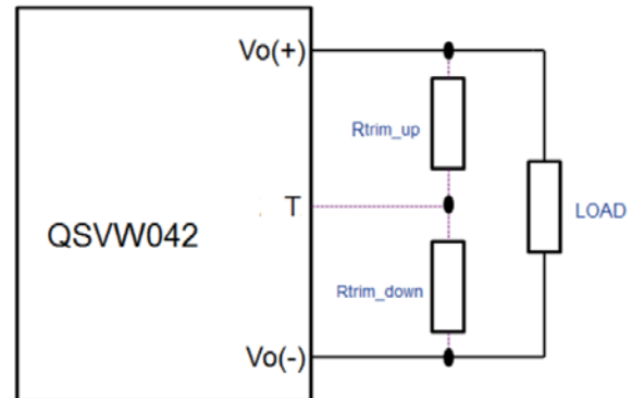
Figure 16. Circuit Configuration to Trim Output Voltage.
