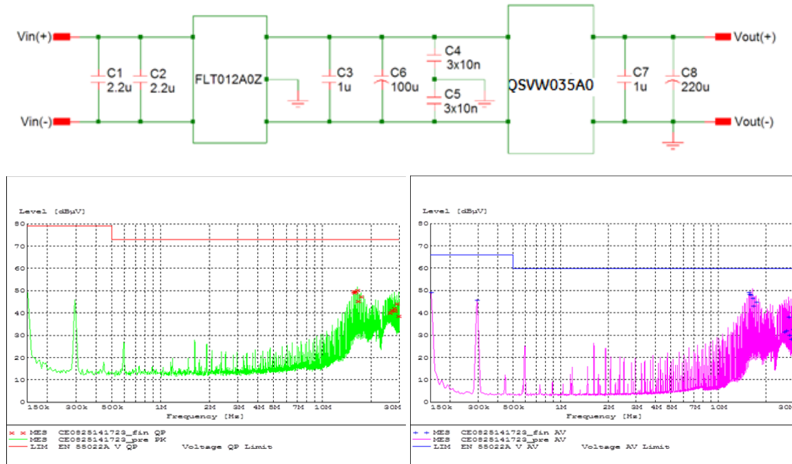
Figure 24. EMC Consideration
