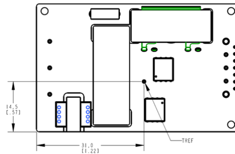
Figure 16. Location of the thermal reference temperature TH .
