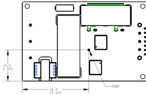
Figure 16. Location of the thermal reference temperature TH_1 .
