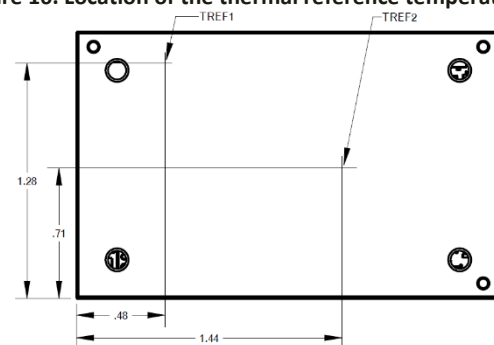
Figure 17. Location of the thermal reference temperature TH_2 for Baseplate module.
