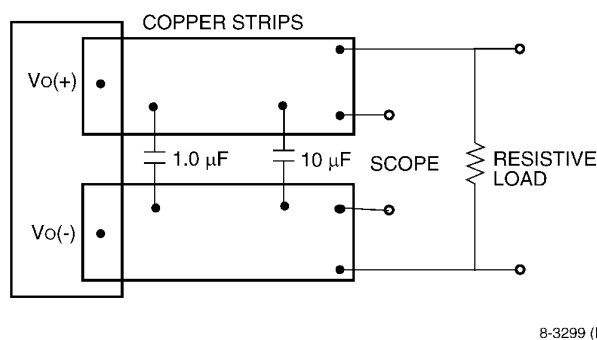
Figure 31. Input Reflected Ripple Current Test Setup.
