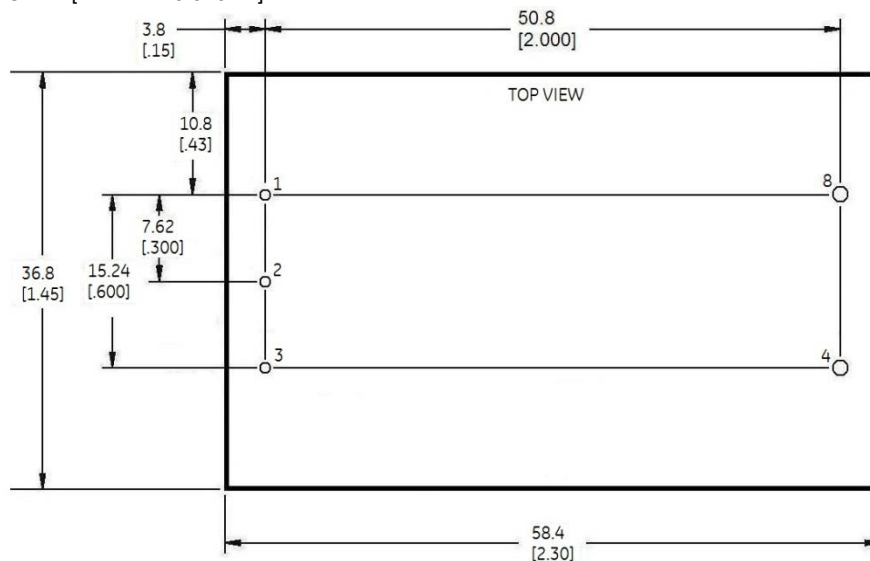
Hole and Pad diameter recommendations:
