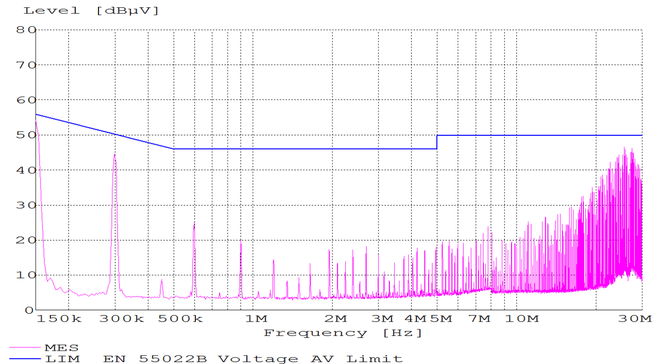
Figure 25. EMC Considerations
