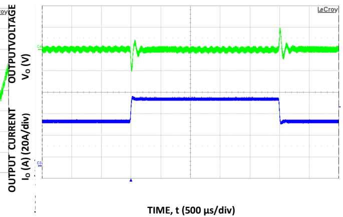
Figure 4. Typical Transient Response to 1.0A/ \mu s Step Change in Load from 50% to 75% to 50% of Full Load, C_o=470\mu F and 50 V dc Input.
