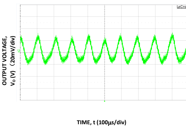
Figure 3. Typical Output Ripple and Noise, I_o = I_{o,max} , C_o=660\mu F .
