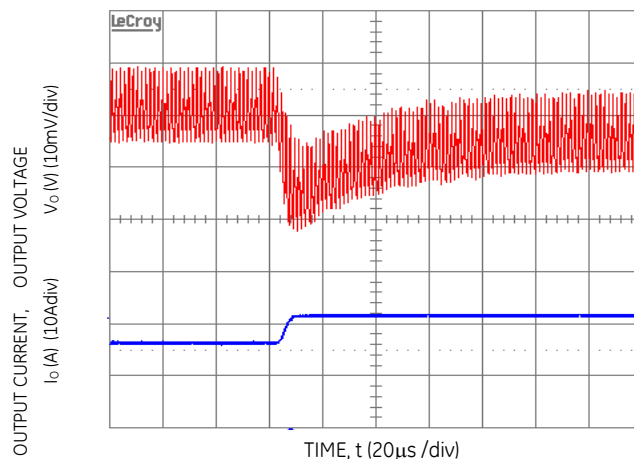
Figure 10. Transient Response to Dynamic Load Change from 50% to 100% at 12Vin, C_{out}=1\times 47\mu\text{F}+3\times 330\mu\text{F} , C_{Tune}=10\text{nF} & R_{Tune}=220\Omega
