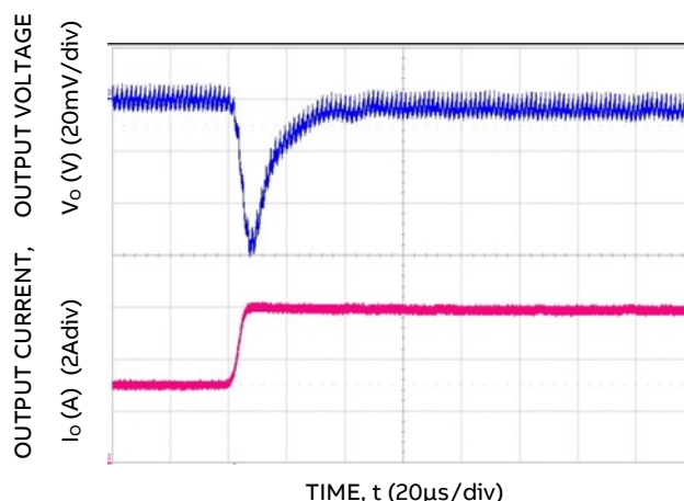
Figure 22. Transient Response to Dynamic Load Change from 50% to 100% at 12V in , C out =3x47μF, C Tune =3300nF, R Tune =178
