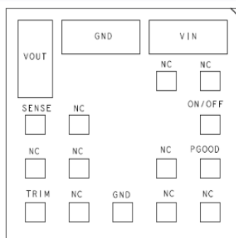
PIN FUNCTION PIN FUNCTION 1 ON/OFF 10 PGOOD 2 VIN 11 NC 3 GND 12 NC 4 VOUT 13 NC 5 VS+ (SENSE) 14 NC 6 TRIM 15 NC 7 GND 16 NC 8 NC 17 NC 9 NC
