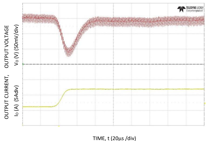
Figure 22. Transient Response to Dynamic Load Change from 50% to 100% at 12Vin, C_{out}=4 \times 47\mu\text{F} + 1 \times 330\mu\text{F} , C_{Tune}=2700\text{p} , RT_{tune}=300
