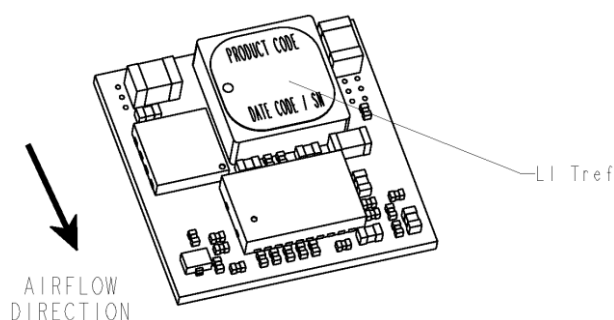
Figure 48. Preferred airflow direction and location of hot-spot of the module ( T_{ref} ).
