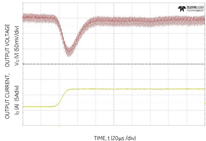
Figure 22. Transient Response to Dynamic Load Change from 50% to 100% at 12Vin, C_{out}=4 \times 47 \mu\text{F} + 1 \times 330 \mu\text{F} , C_{Tune}=2700\text{pF} , R_{Tune}=300\Omega
