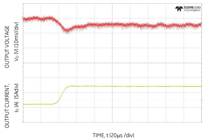
Figure 4. Transient Response to Dynamic Load Change from 50% to 100% at 12Vin, C_{out}=4 \times 47\mu\text{F} + 6 \times 330\mu\text{F} , C_{Tune}=47\text{nF} , R_{Tune}=300
