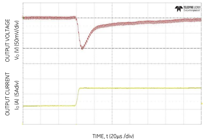
Figure 34. Transient Response to Dynamic Load Change from 50% to 100% at 12Vin, C_{out}=6 \times 47\mu\text{F} , C_{Tune}=1200\text{pF} , RT_{tune}=300
