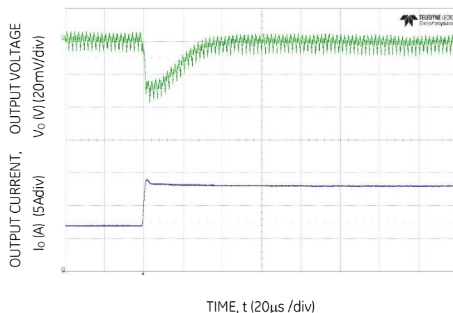
Figure 16. Transient Response to Dynamic Load Change from 50% to 100% at 12V in , C_{out}=8\times 47\mu\text{F}+2\times 330\mu\text{F} , C_{Tune}=1.8\text{nF} , R_{Tune}=300\Omega
